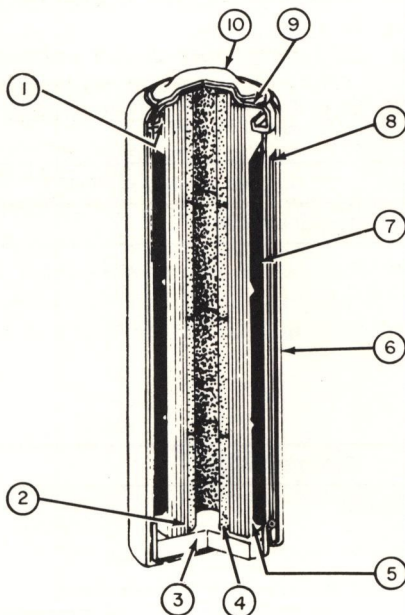
Fig. 5. Cross Section of a Typical Cylindrical Zinc-Mercuric Oxide Dry Cell.
