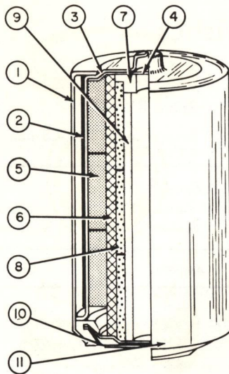
Fig. 6. Cross Section of a Typical Cylindrical Zinc-Manganese Dioxide Dry Cell.
