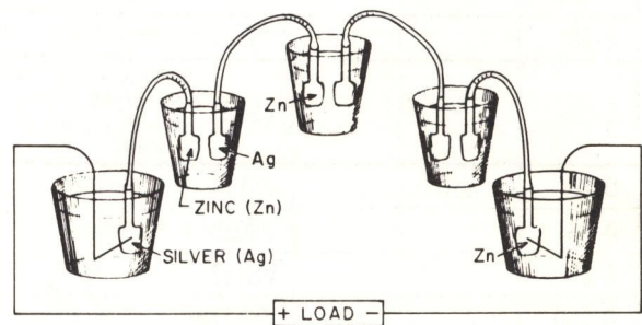
Fig. 2. Volta's Crown of Cups.
