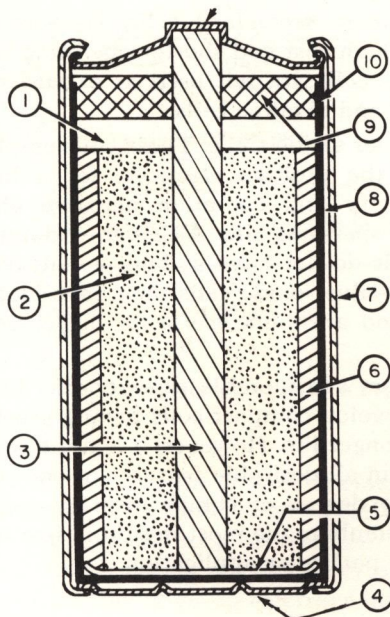
Fig. 4. Cross Section of a Typical Cylindrical Zinc-Carbon Dry Cell.
