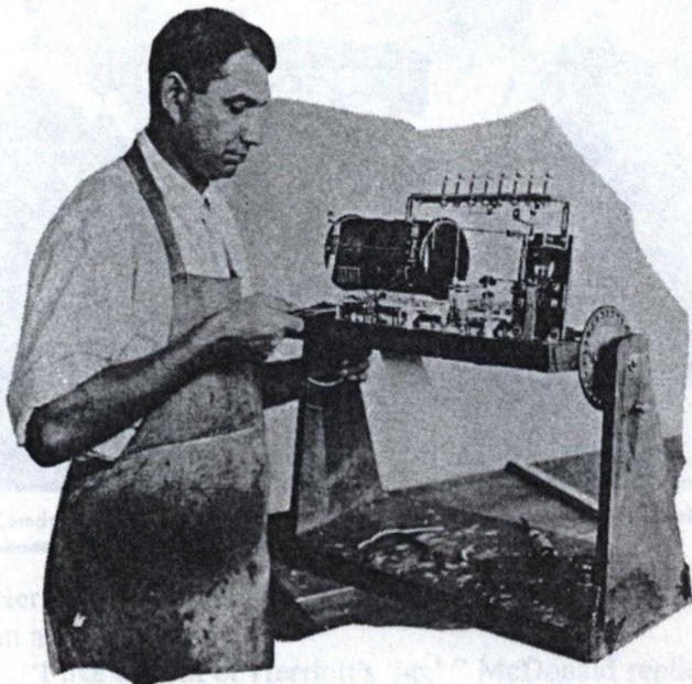
Before development of assembly line methods, sets were built one at a time. 1922 Chicago Radio Laboratory, Kedzie Ave. factory scene.
