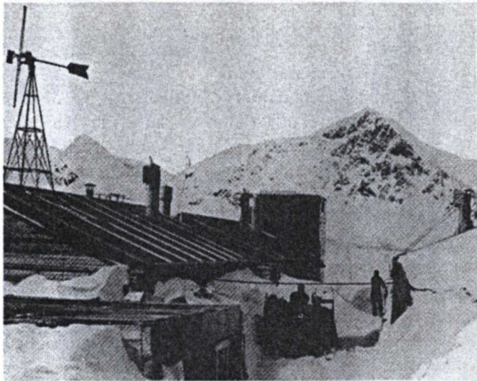
Harnessing wind throughout the world, Wincharger installations like this one in Iceland brought electricity to remote areas.
