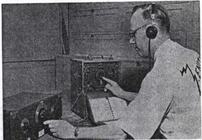
Mass production of sensitive frequency meter was one of Zenith's major contributions to World War II.
