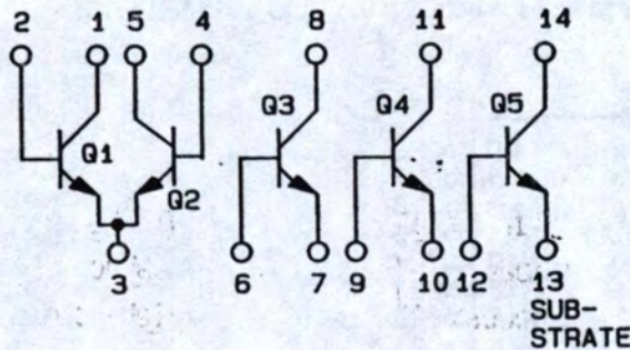
FIG. 1 SCHEMATIC DIAGRAM
