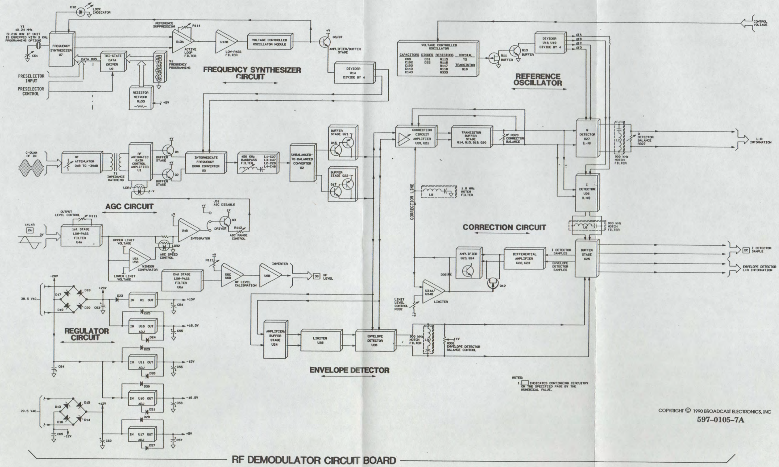
FIGURE 4-1. AS-10 SIMPLIFIED SCHEMATIC (Sheet 1 of 3)
