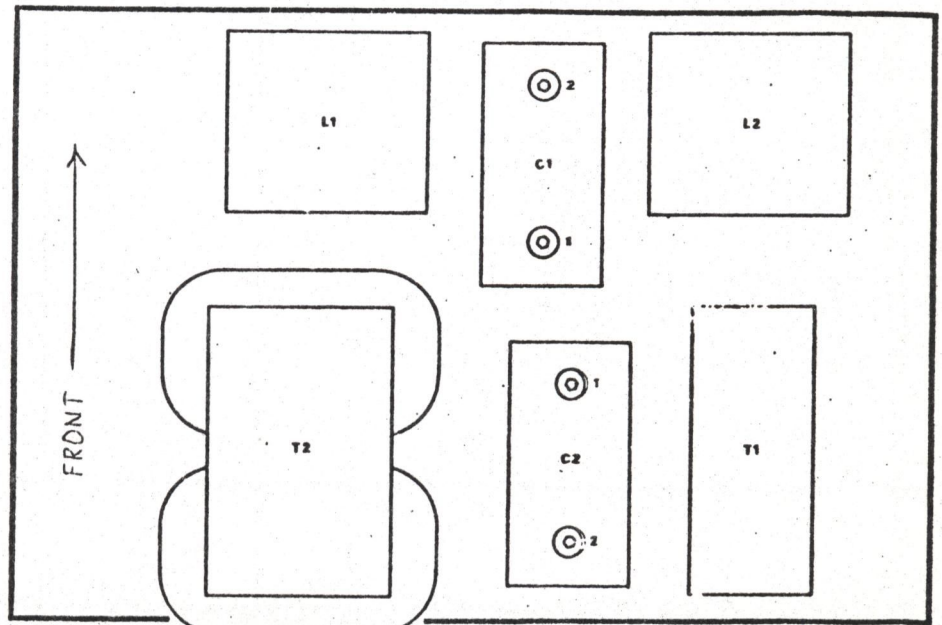
831D-2 , BOTTOM SECTION , TOP VIEW
