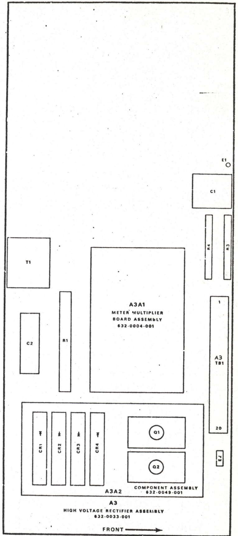
831D-2 , RIGHT SIDE
