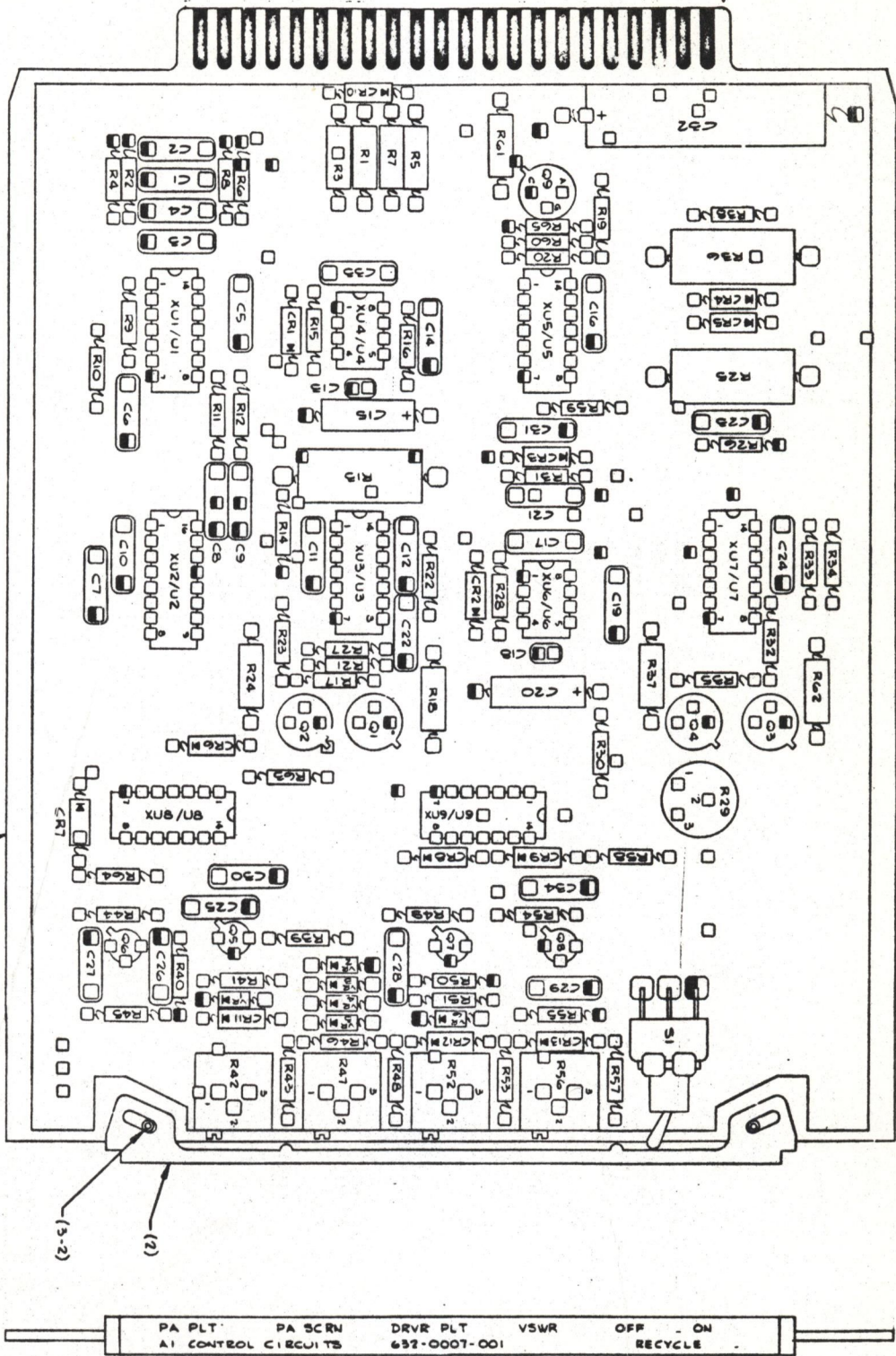
A1A1 CONTROL CIRCUITS CPN 632-0007-001
