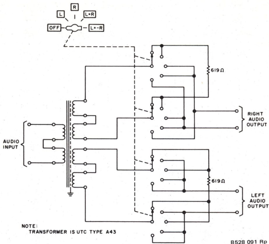
Figure 5-3. Stereo Test Circuit, Schematic Diagram.
