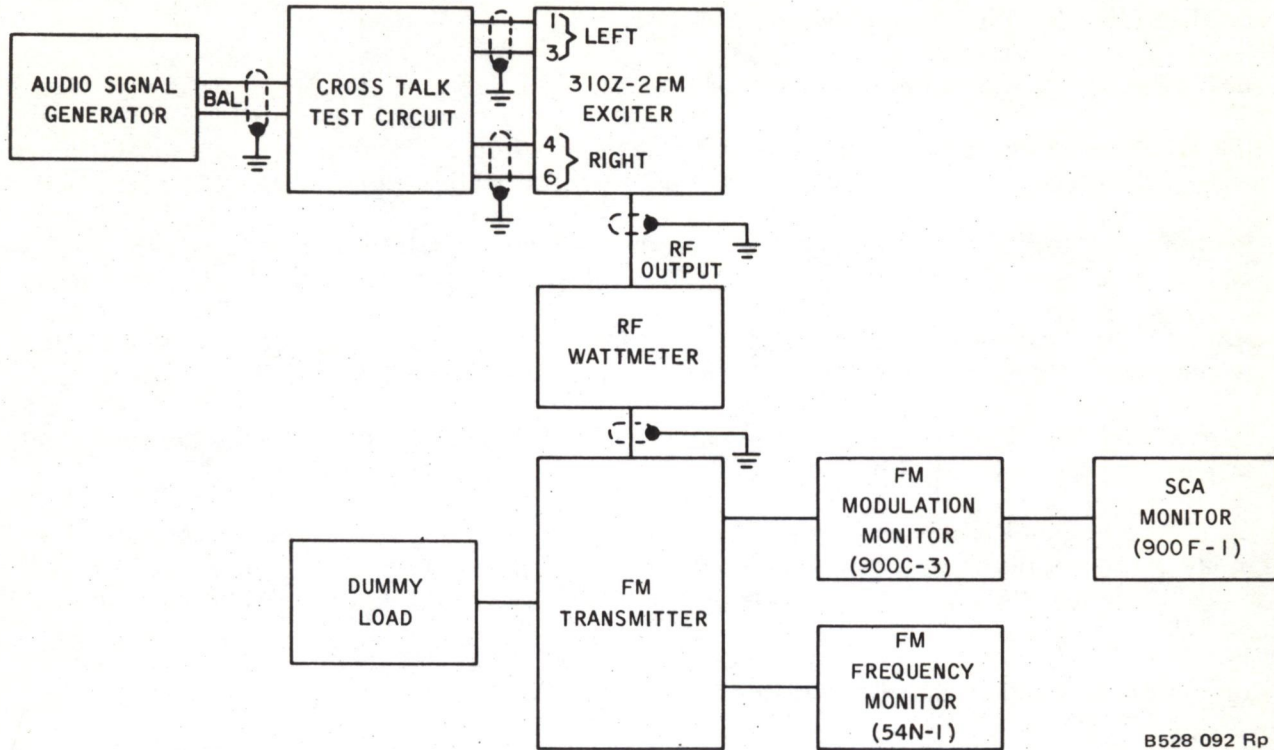
Figure 5-4. Test Equipment Connections to 310Z-2 for Crosstalk Test.
