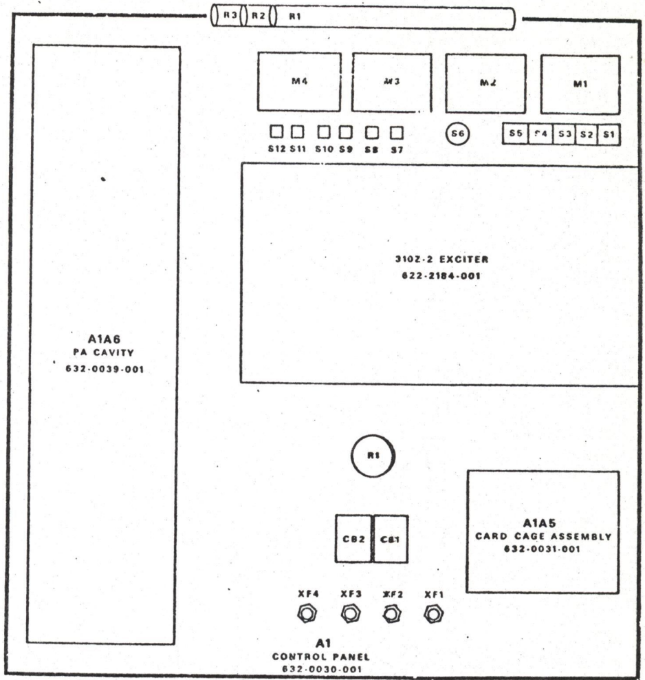
831D-2 , FRONT PANEL , BACK VIEW
