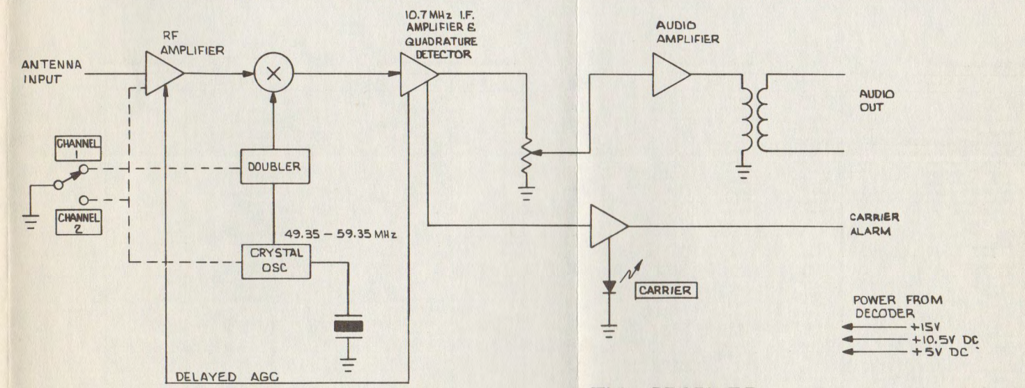
FM RECEIVER
