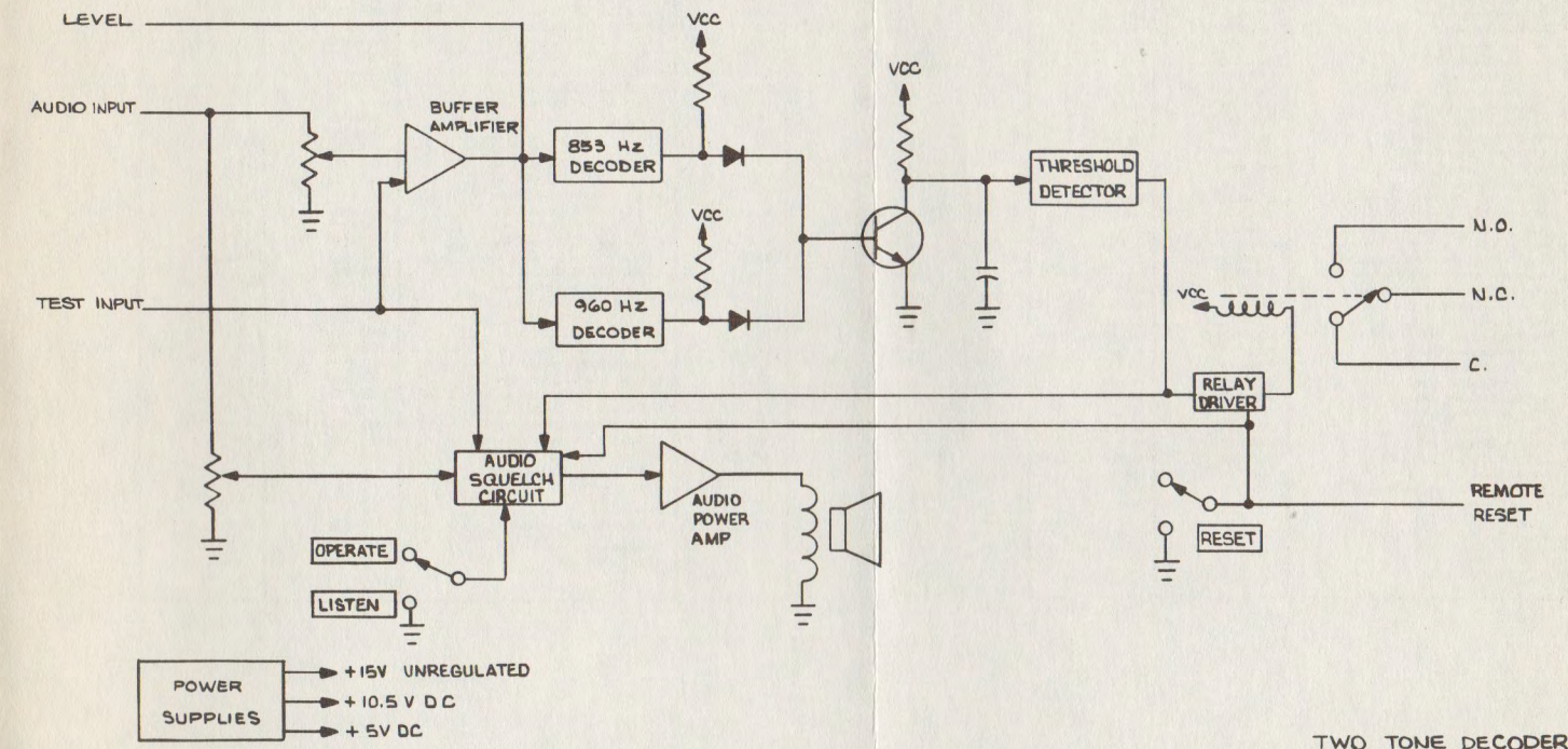
TWO TONE DECODER
