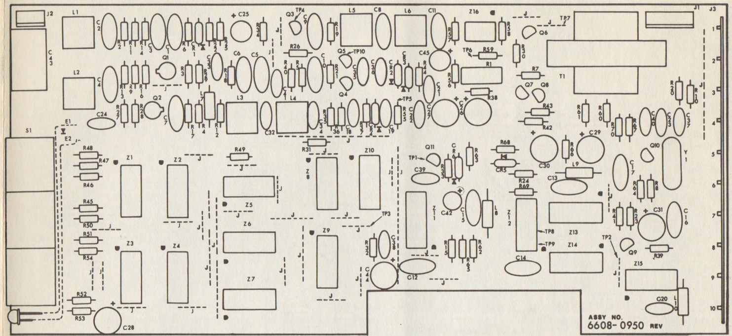
AM RECEIVER
